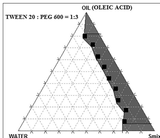
Figure 3: Ternary plot of Tween 20: Polyethylene glycol 600 = 1:3
