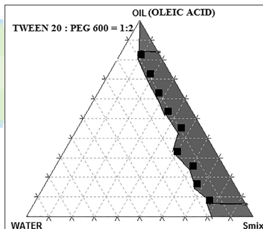
Figure 2: Ternary plot of Tween 20: Polyethylene glycol 600 = 1:2
