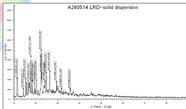
Figure 3: X-ray powder diffraction of hydrotropic solid dispersion of LRD
