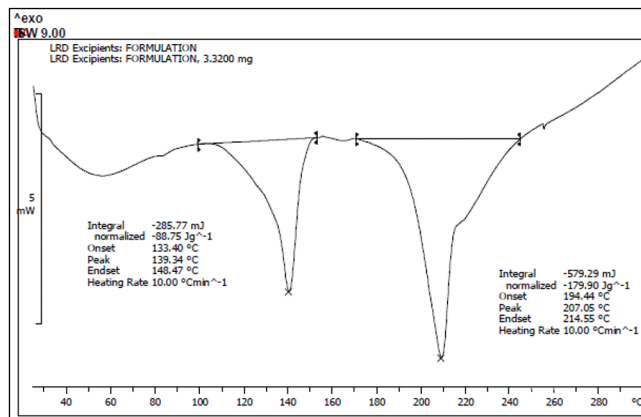
Figure 5: Differential scanning calorimetry of physical mixture of LRD and hydrotropic solid dispersion
