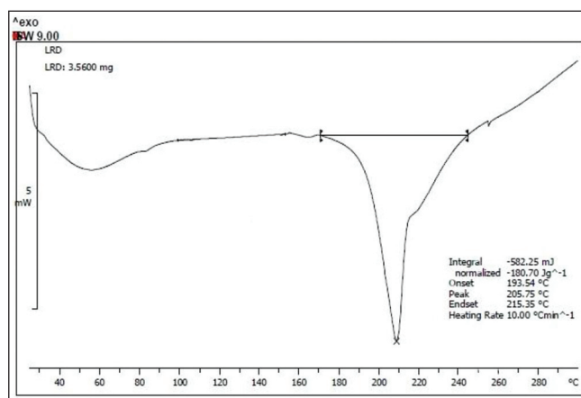
Figure 4: Differential scanning calorimetry thermogram of LRD
