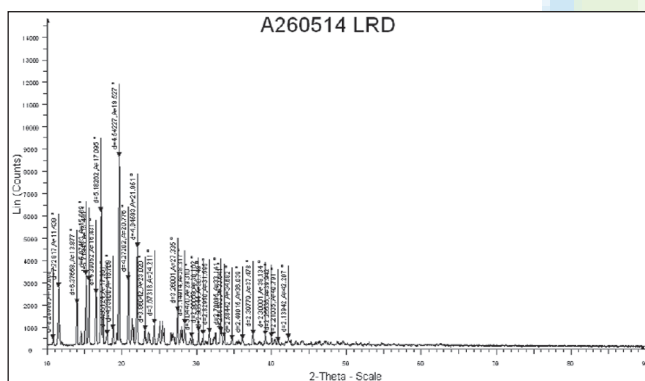
Figure 2: X-ray powder diffraction spectra of LRD
