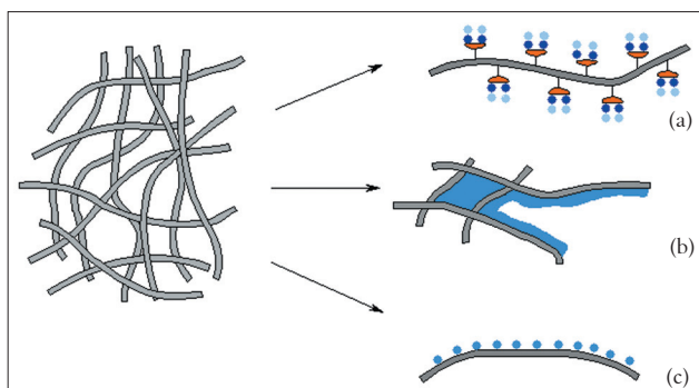
Figure 2: Possible association of water with the polymer molecules; (a) water molecules strongly attached to the polar groups of the polymer chains by hydrogen-bonds in two layers; (b) microscopic voids inside the polymer filled with excess water; (c) individual water molecules attached to the non-polar region of the polymer by weak interaction forces
