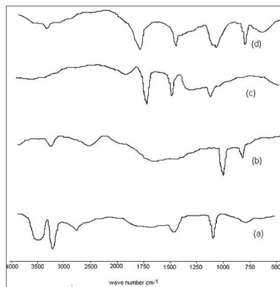
Figure 2: FTIR spectrographs of (a) \beta -CD, (b) CL \beta -CD, (c) pravastatin sodium, and (d) PS-loaded CL \beta -CD
